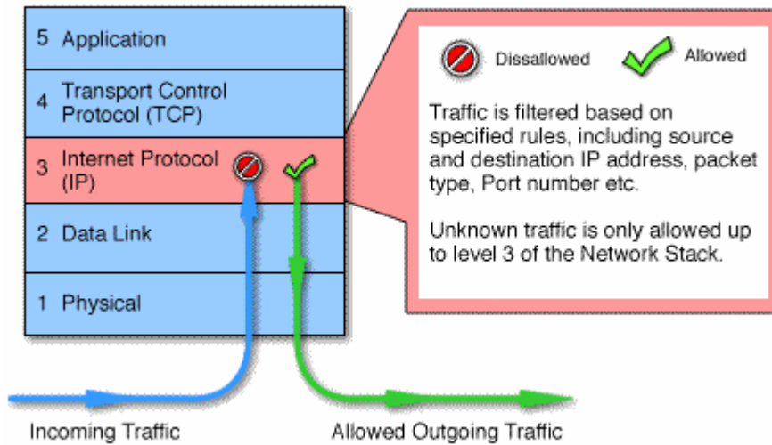
Figure 4: Packet Filtering Firewall
